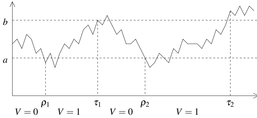
Figure 2: Illustration of the sequence of stopping times introduced in Definition 8.25.
