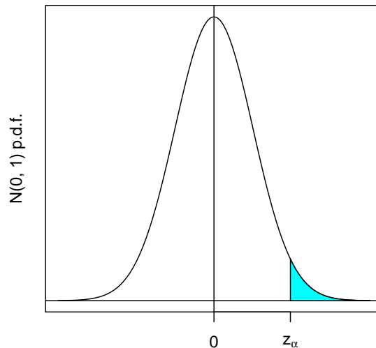
Figure 5.2. Standard normal p.d.f.: the shaded area, i.e. the area under the curve to the right of z_\alpha , is \alpha .
