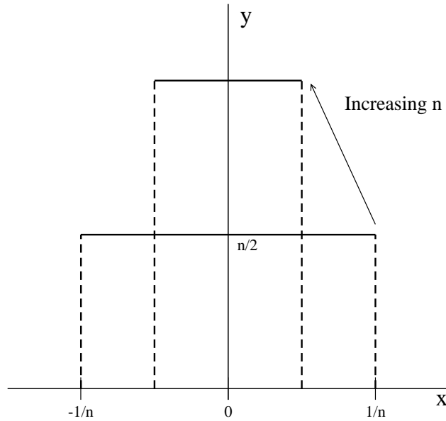
Figure 2: Hat functions, see equation (44).
