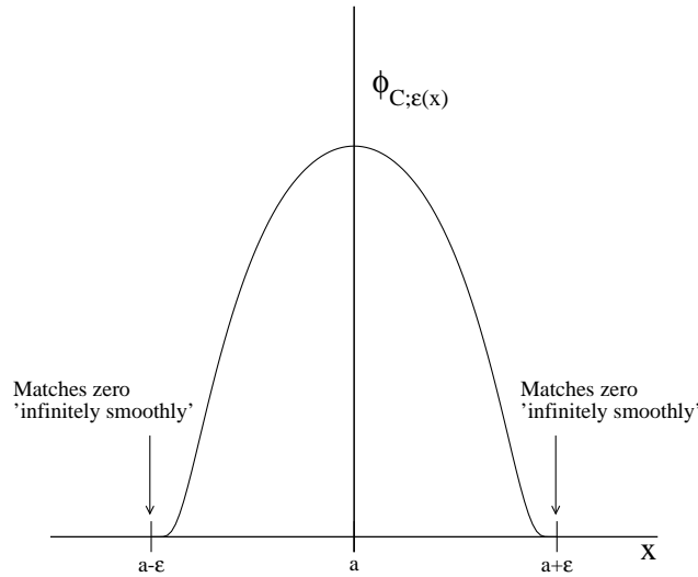
Figure 3: Sample test function, corresponding to (72)
