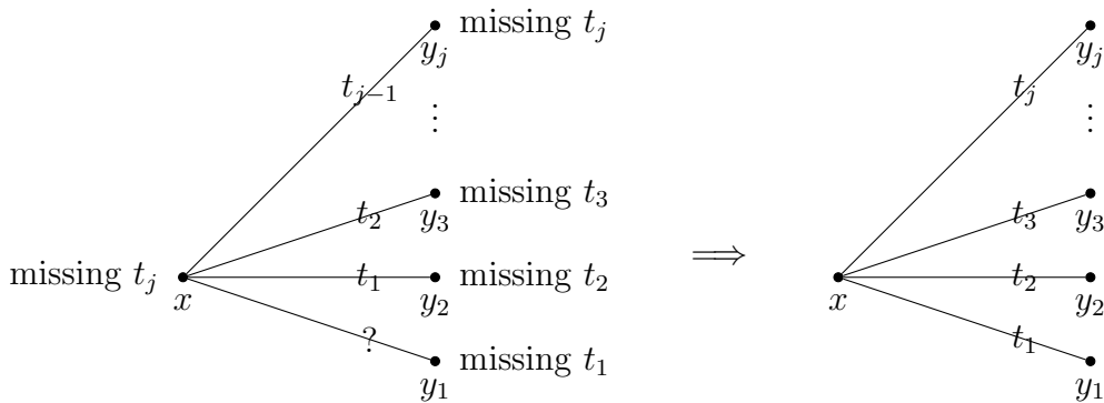
Figure 6: Recolouring a fan when some t_j is missing at x .
