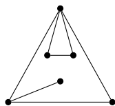
Figure 9: A plane graph with three faces.
