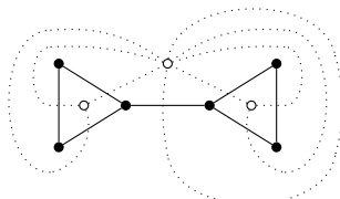
Figure 10: A planar graph and its dual. The dual is a multigraph.
