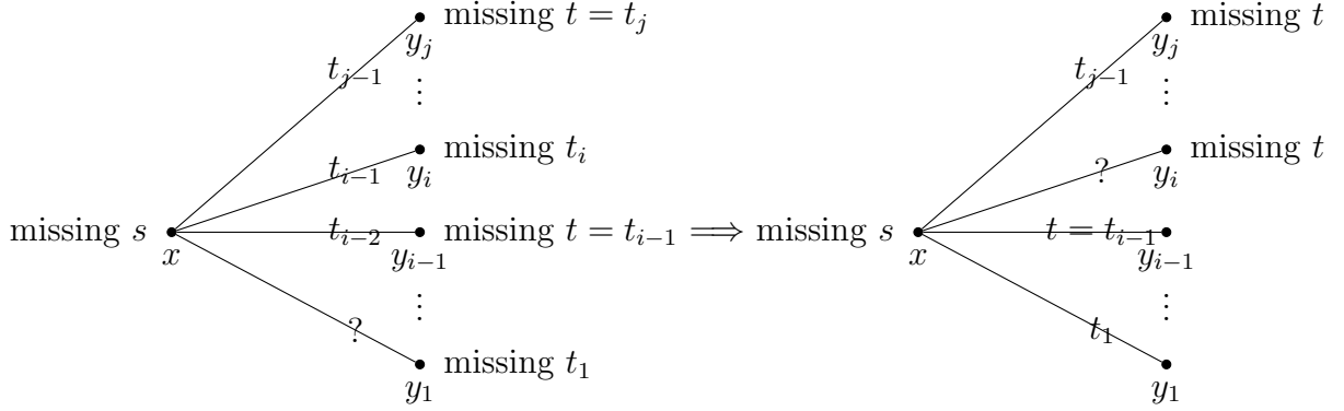
Figure 7: Recolouring a fan when some t = t_j = t_{i-1} .
