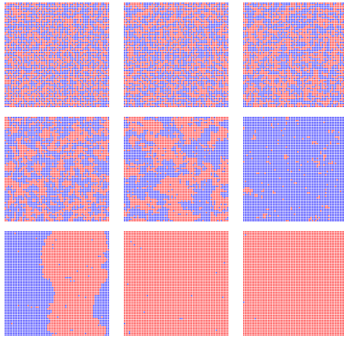
Typical states with \beta = 0.0, \dots, \beta = 0.8
