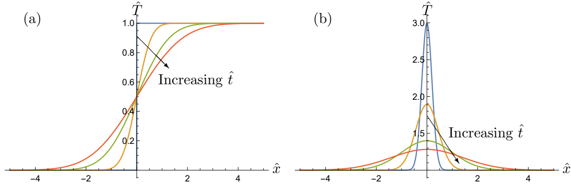
Figure 1.3: Similarity solution for the heat equation with (a) \hat{T}_{-\infty} = 0 , \hat{T}_{+\infty} = 1 and D = 1 for times t = 0, 0.1, 0.5, 1 ; (b) \hat{T}_{-\infty} = 0 , \hat{T}_{+\infty} = 0 and D = 1 for times t = 0.02, 0.1, 0.5, 1
