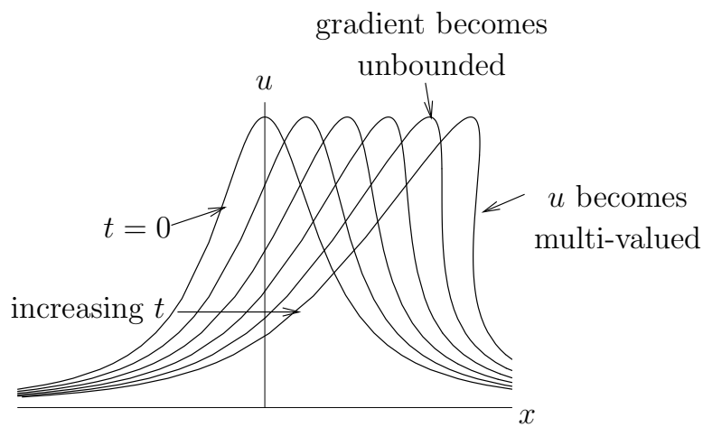
Figure 4.4: Schematic of a steepening simple wave.
