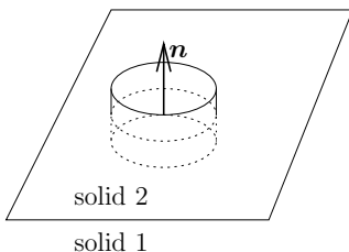
Figure 1.4: Schematic of a small pill-box-shaped region at the boundary between two elastic solids.
