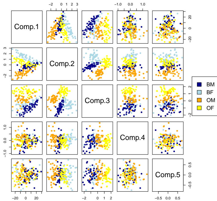
Figure 17: Pairs plot of PC components for the Crabs dataset.
