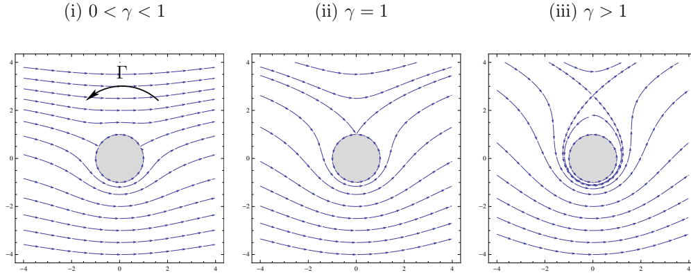
Figure 2.15: Streamlines for uniform flow at speed U flow past a cylinder of radius a with circulation \Gamma . (i) 0 < \gamma < 1 ; (ii) \gamma = 1 ; (iii) \gamma > 1 , where \gamma = \Gamma/4\pi Ua .
