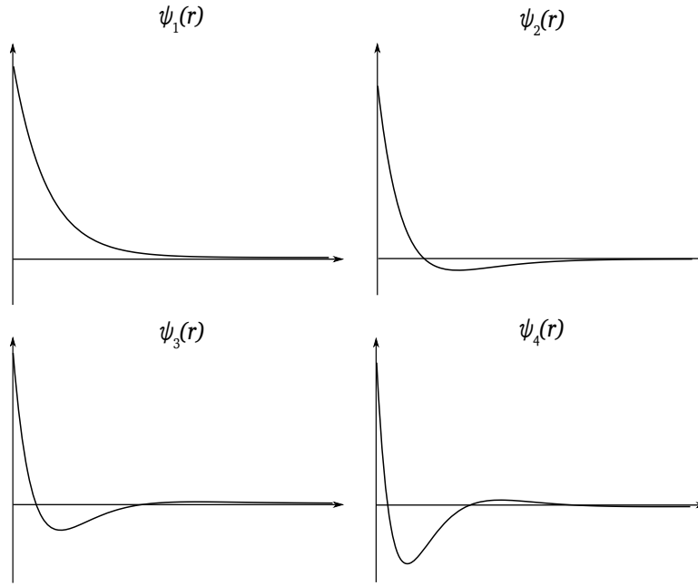
Figure 11: The ground state and first three spherically symmetric excited state wave functions \psi_N(r) \equiv \psi_{N,0,0}(r) of the hydrogen atom.
