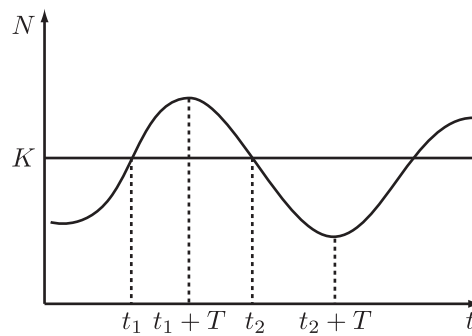
Figure 2.1: Schematic of the oscillatory nature of solutions.
