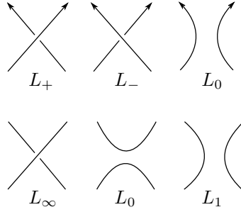
FIGURE 16. The top row shows the three links featuring in the oriented skein relation, and the bottom row the links in the unoriented skein relation.
