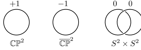
FIGURE 17. Kirby diagrams for \mathbb{CP}^2 , \overline{\mathbb{CP}}^2 , and S^2 \times S^2 .
