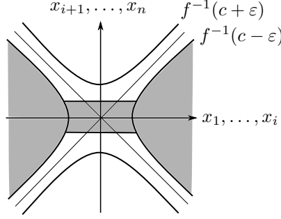
FIGURE 1. This figure shows the level sets f^{-1}(c - \varepsilon) , f(c) , and f^{-1}(c + \varepsilon) of the function f in Lemma 1.5.2, where c = f(0) . The shaded region is M^{c-\varepsilon} union the i -handle D^i \times D^{n-i} , which becomes diffeomorphic to M^{c+\varepsilon} after smoothing the corners.
