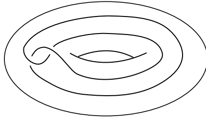
FIGURE 13. The Whitehead knot in the solid torus.
