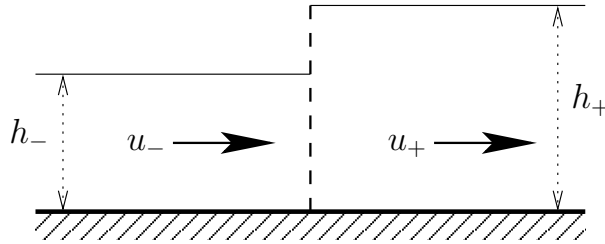
Figure 5.7: Schematic of a hydraulic jump.
