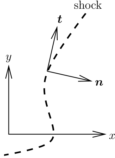
Figure 5.10: Schematic of a curved shock with local axes in the normal and tangential directions.
