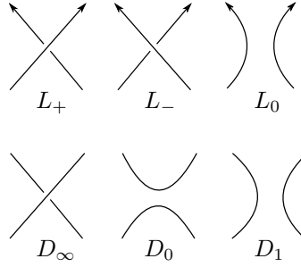
FIGURE 16. The top row shows the three links featuring in the oriented skein relation, and the bottom row the diagrams in the unoriented skein relation.
