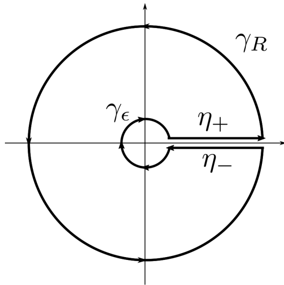
Figure 3.3: A keyhole contour.
