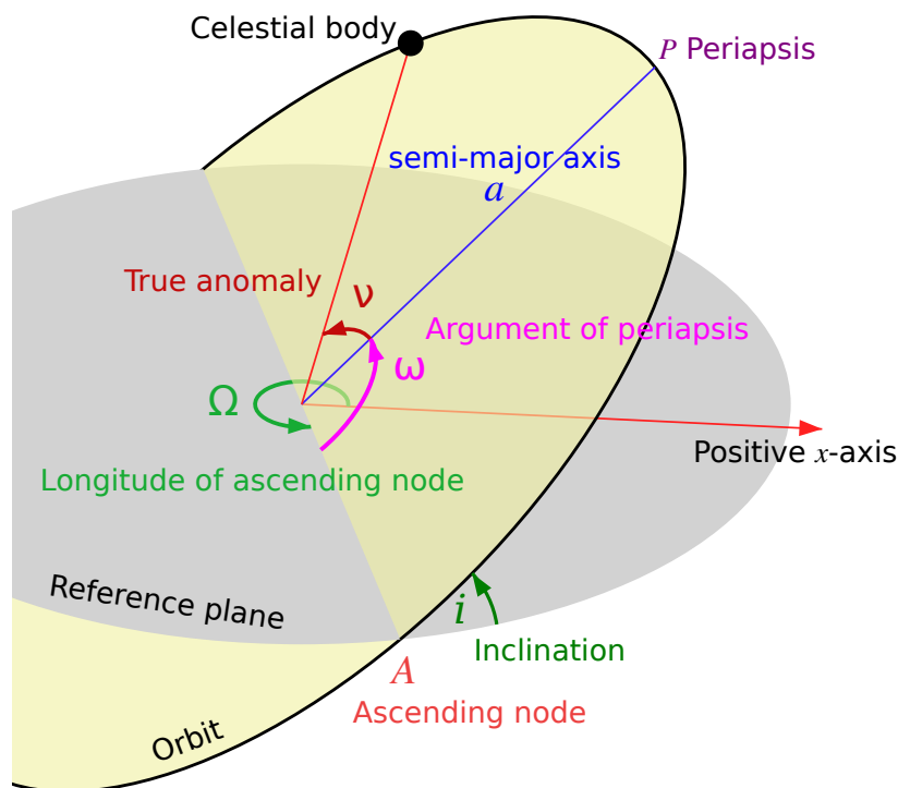
Figure 21.1: The Keplerian orbital elements. Credit: modified from wikipedia .
