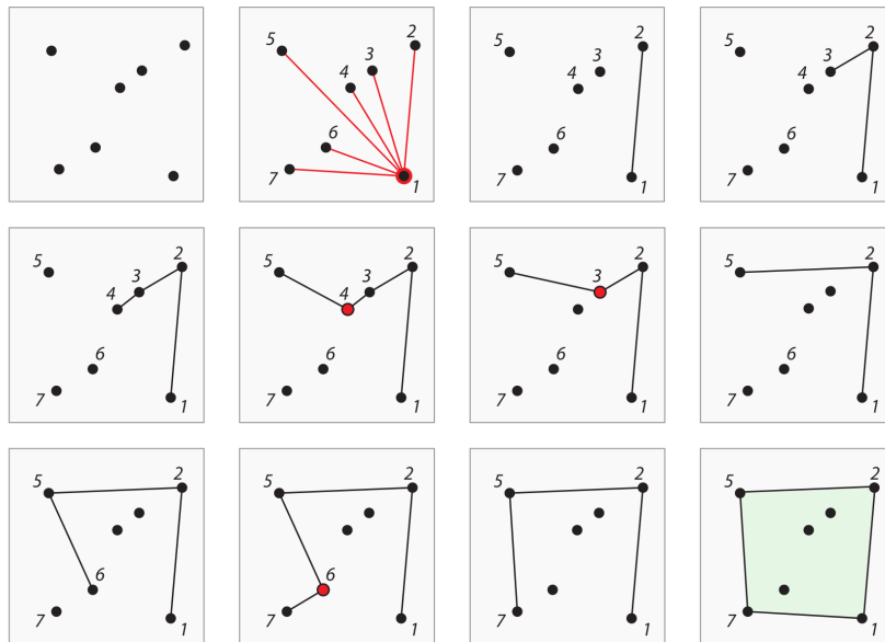
Figure 20.4: Steps of the Graham scan. The points are sorted in order from the base point b (labelled 1). In the 6 th panel, the three vertices 3-4-5 form a right turn, so 4 cannot be in the convex hull. In the 7 th panel, the three vertices 2-3-5 also form a right turn, so 3 also cannot be in the convex hull.
