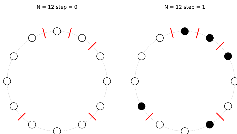
Figure 19.1: Initial configuration of a Kac ring (left) and the state after one step (right). Marked edges are shown in red.
