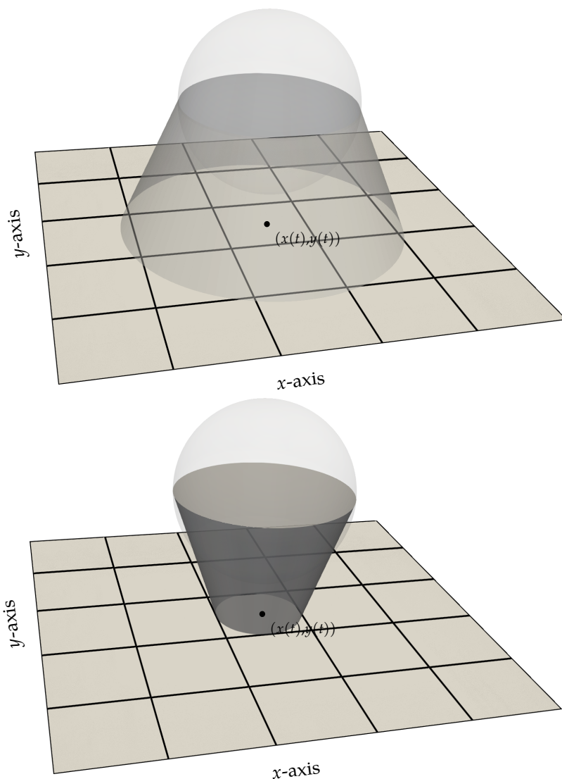
Figure 18.4: An illustration of some of the Besselian elements. The Moon (transparent sphere) casts a penumbral shadow (top), where some of the Sun's light is blocked and the eclipse will be partial, and an umbral shadow (bottom), where all of the Sun's light is blocked and the eclipse will be total. By construction, the fundamental plane (the grid) is normal to the cones and their projections onto the fundamental plane are disks. The centre of the disk is (x(t), y(t)) . The radius of the penumbral disk on the fundamental plane is l_1(t) and the radius of the umbral disk is |l_2(t)| . The normal to the plane is described by d(t) and \mu(t) .
