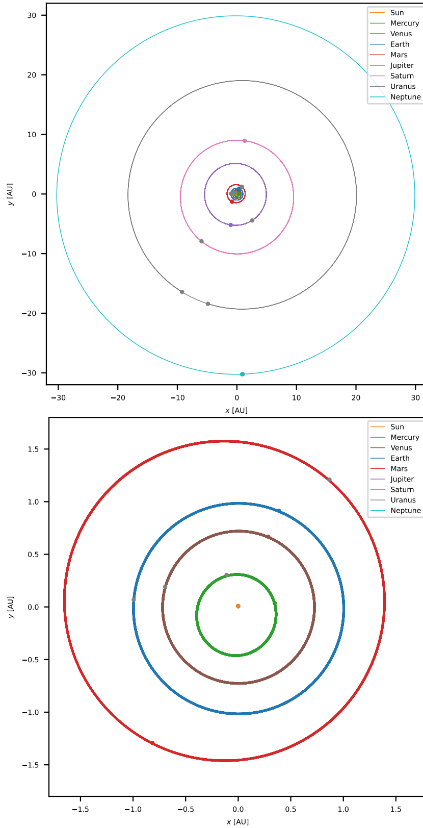
Figure 13.2: A simulation of the solar system over one Neptunian year, code blocks 13.2 to 13.5 . The lower figure zooms in to the rocky inner planets.
