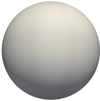
(a) a solid sphere, (b_0, b_1, b_2) = (1, 0, 0)
