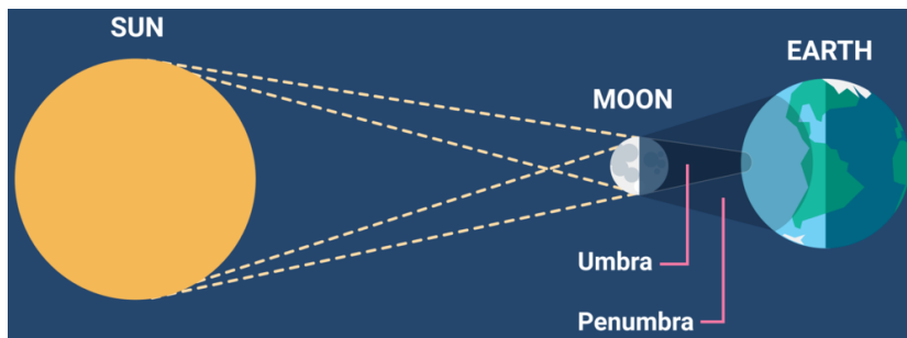
Figure 18.3: The umbral and penumbral cone of a solar eclipse. Credit: timeand-date.com .
