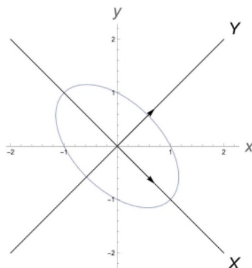
Figure 1: x^2 + xy + y^2 = 1
