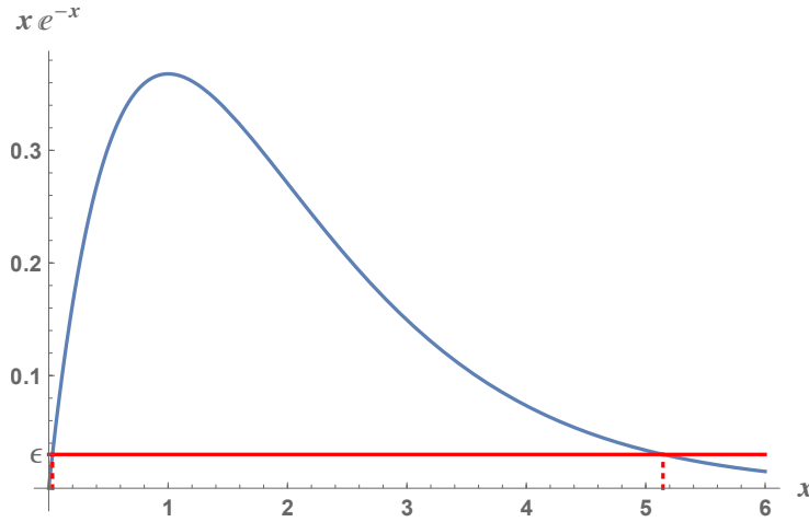
Figure 7.1: The function x e^{-x} plotted versus x , indicating two roots to equation (7.39) with 0 < \varepsilon \ll 1 .
