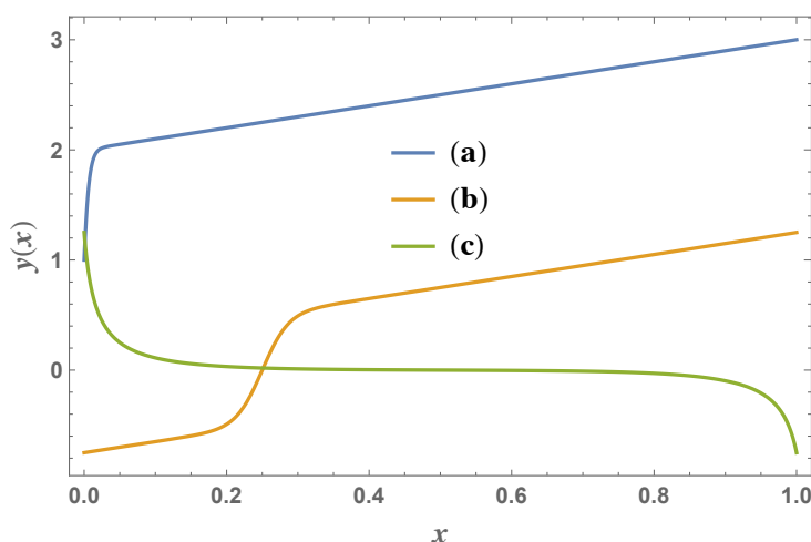
Figure 8.3: Solutions of the ODE (8.53) satisfying each of the boundary conditions (8.54), computed with \varepsilon = 0.01 .
