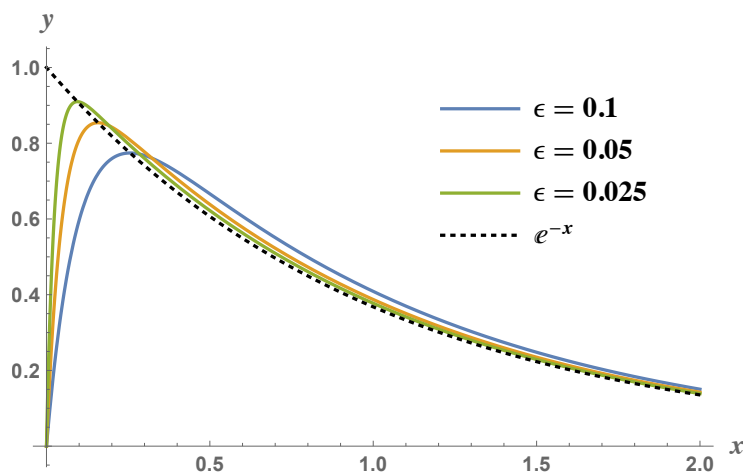
Figure 8.1: The function y(x; \varepsilon) given by (8.24) plotted versus x with three different values of \varepsilon . The leading-order outer solution e^{-x} is plotted as a black dotted curve.
