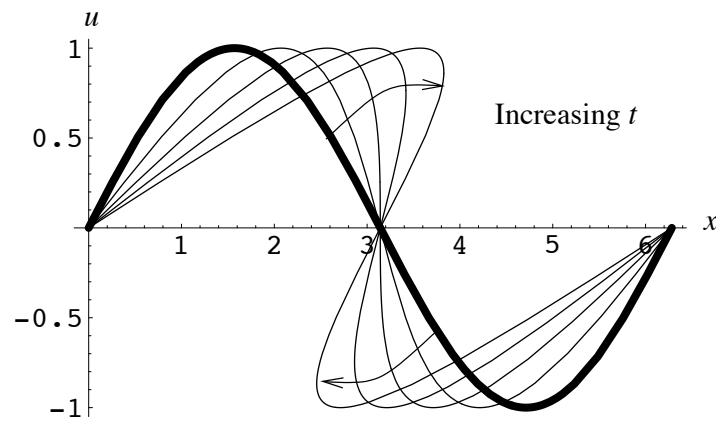
Figure 2.7: The solution u(x, t) from Example 2.10 plotted versus x for t = 0.5, 1.0, 1.5, 2.0 . The initial solution u(x, 0) = \sin(x) is shown as the thicker line.
