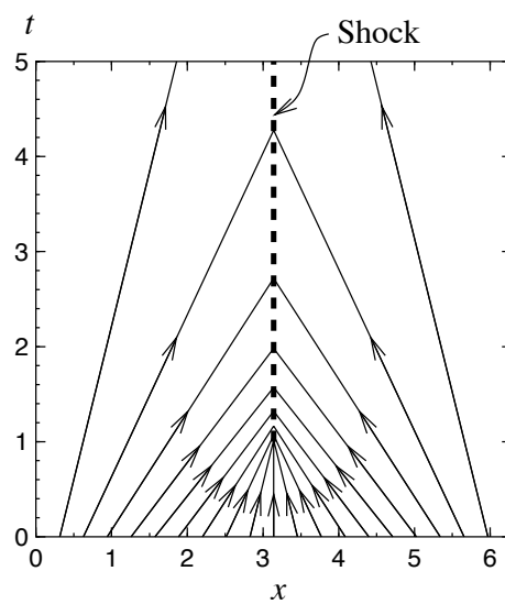
Figure 3.5: Characteristic projections and shock for Example 3.6.
