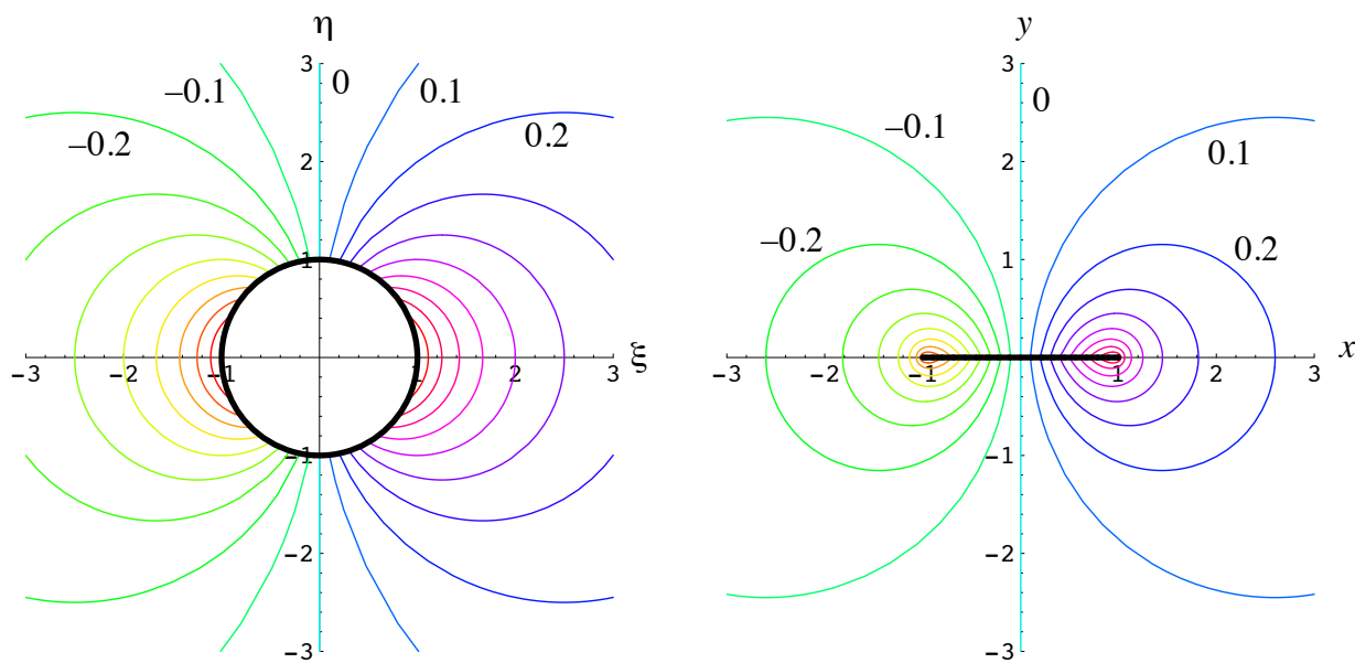
Figure 8.1: Contour plots of the solution u given by (8.68) versus \xi = \Re(\zeta) and \eta = \Im(\zeta) (left plot); x and y (right plot). The contour values are u = -0.9, -0.8, \dots, 0.8, 0.9 .
