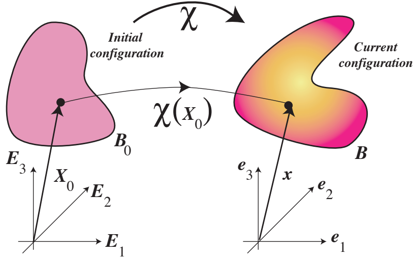
Figure 30: Basic kinematics of nonlinear elasticity. Two configurations are defined (with possibly different sets of coordinates). The deformation is a 1-1 map between points of the reference configuration \mathcal{B}_0 and points of the current configuration \mathcal{B} .
