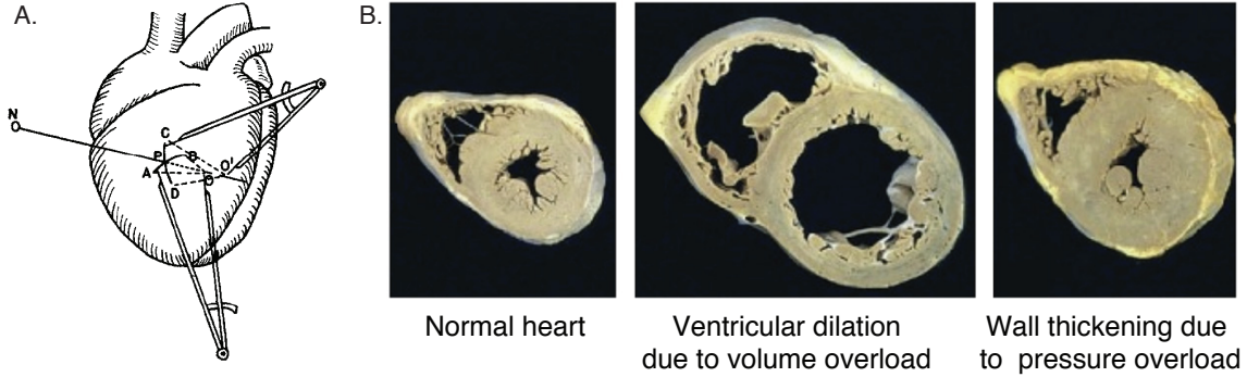
Figure 11: Growth and remodelling in the heart: A. Observation of the principal radii of curvature on the heart surface as originally performed by Woods [64]. (B) Pathology of the heart leading to increase in size. Left: normal heart, middle: ventricular dilation due to volume overload, right: increase in wall thickness due to pressure overload [65] Reproduced WITHOUT permission.
