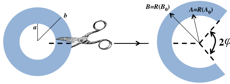
Figure 36: Schematic of a radial cut in a ring and the corresponding opening angle \varphi .
