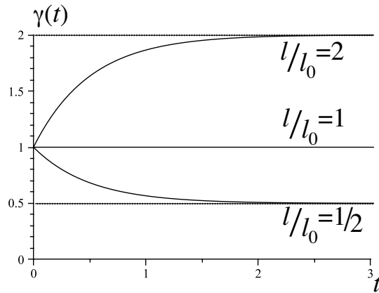
Figure 24: Growth evolution of a filament with homeostatic stress \sigma^* of length l_0 either extended to a filament of length l = 2l_0 or compressed to a filament of length l = l_0/2 ( \sigma^* = 1 ).
