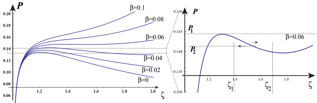
Figure 15: Behavior of a tube under pressure and axial force for a Fung material ( \beta > 0 ). Parameters for all figures: A = 1, B = 1.2, \mu = 1, F = 0.1, \chi = 1 .
