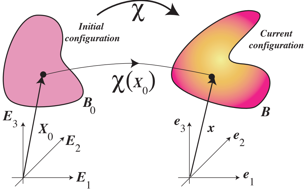
Figure 3: Basic kinematic of nonlinear elasticity. Two configurations are defined. The deformation is a 1-1 map between points of the reference configuration \mathcal{B}_0 and points of the current configuration \mathcal{B} .
