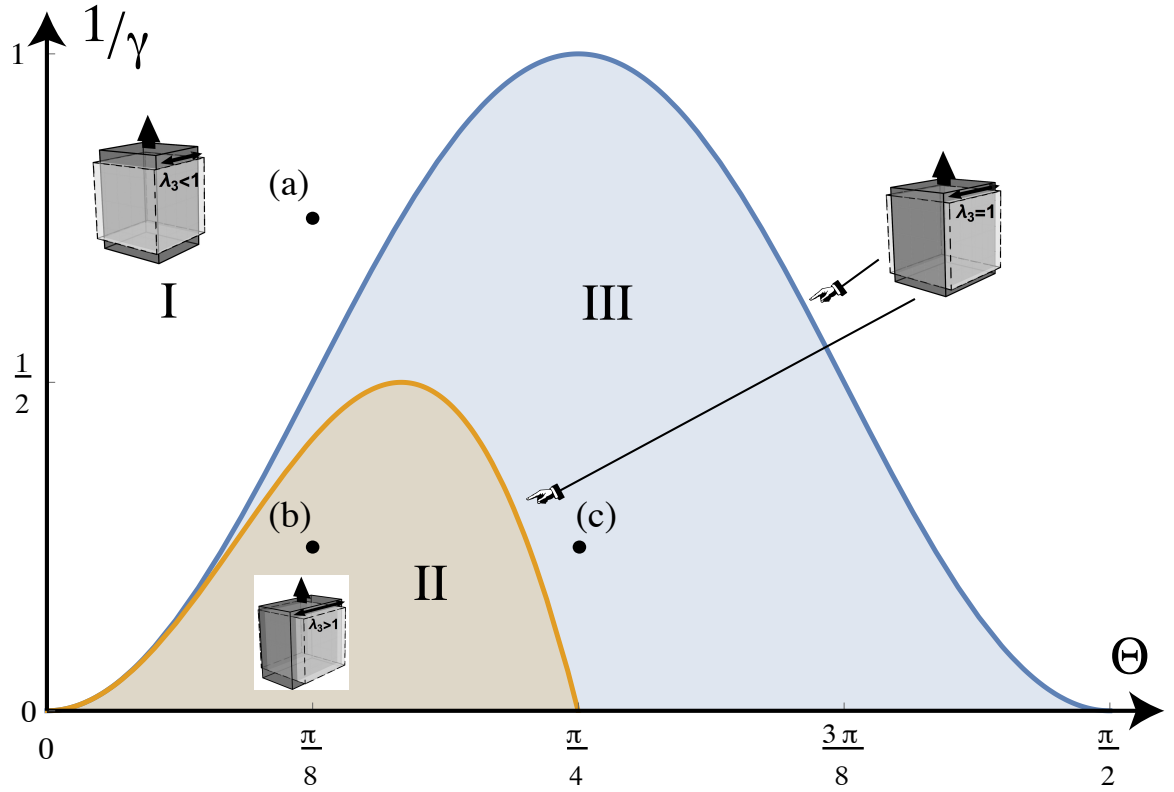
Figure 29: Parameter space for inversion: depending on the relative fiber stiffness \gamma and the fiber direction \Theta , in tension, the thickness of a fiber either decreases (Zone I), increases (Zone II), or first decreases, then increases (Zone III). Insert shown for different values of the tension. The stretch profiles as a function of the tension for specific points (a,b,c) are given in Figure 28.
