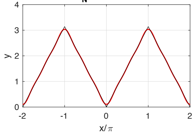
S_N(x) for N = 8
