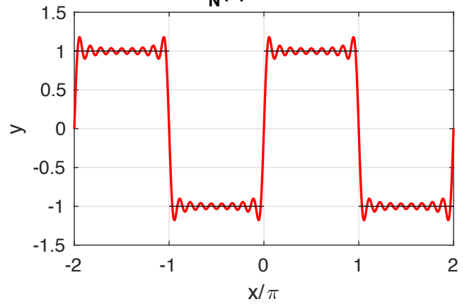
S_N(x) for N = 32
