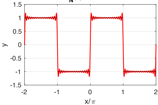
S_N(x) for N = 16
