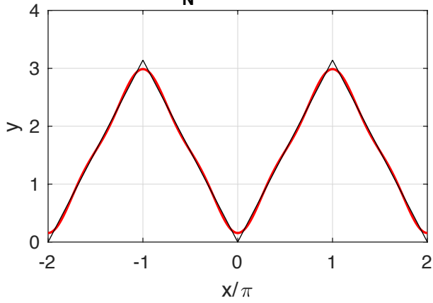
S_N(x) for N = 4
