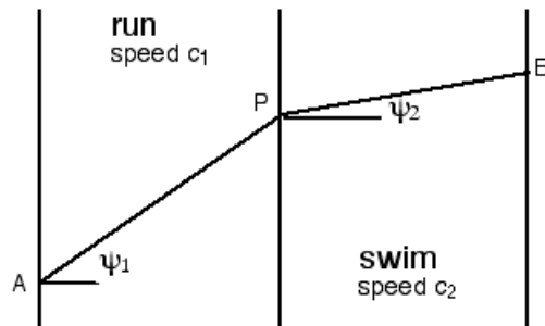
Figure 2: The biathlon problem
