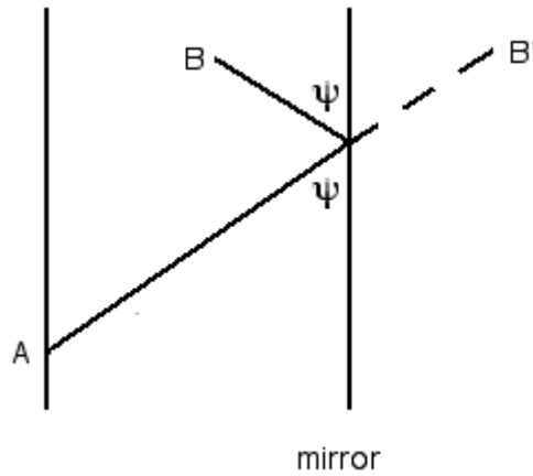
Figure 1: The shortest path from A to B
